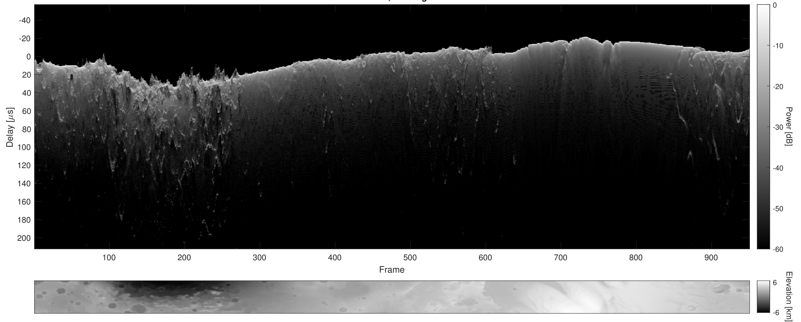
Orbit 21389, Cluttergram
