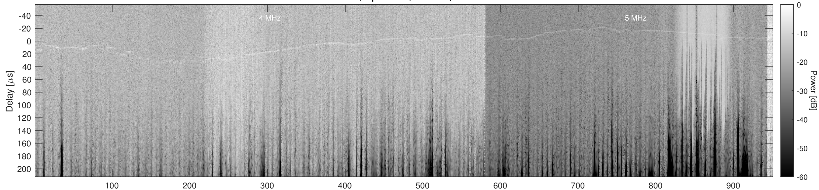
Orbit 21389, Optimized, Window, Channel 2
