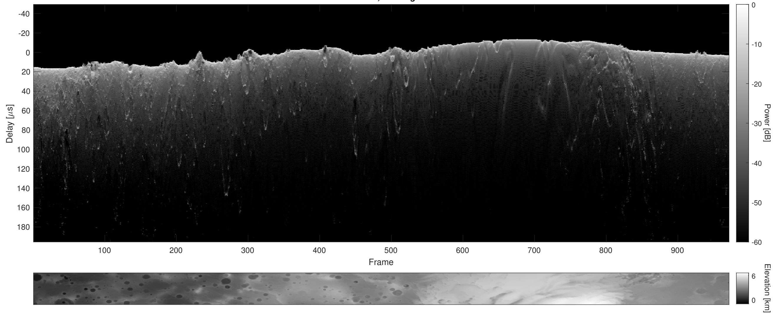
Orbit 21395, Cluttergram
