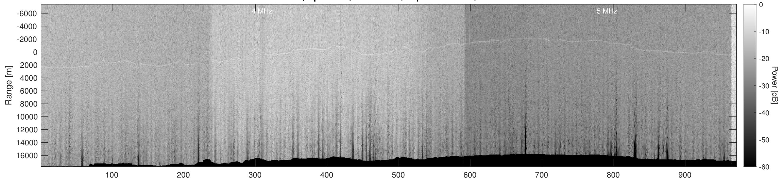
Orbit 21395, Optimized, No Window, Depth-Corrected, Channel 2
