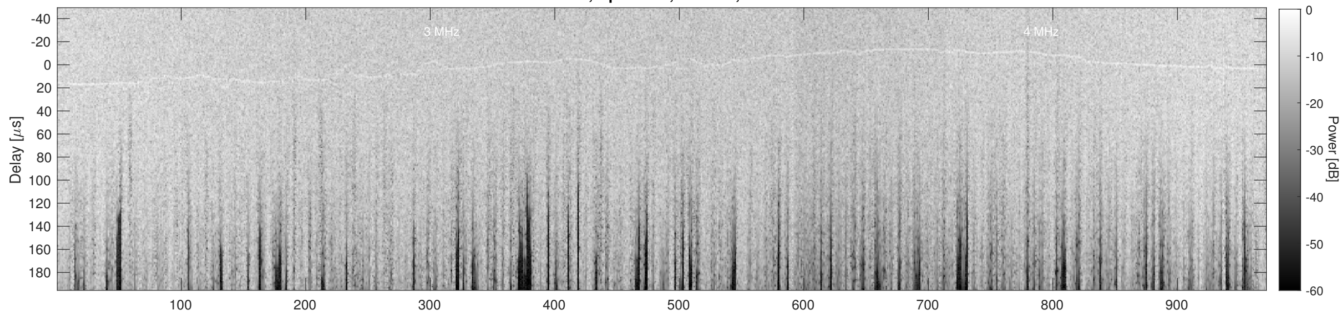
Orbit 21395, Cluttergram
