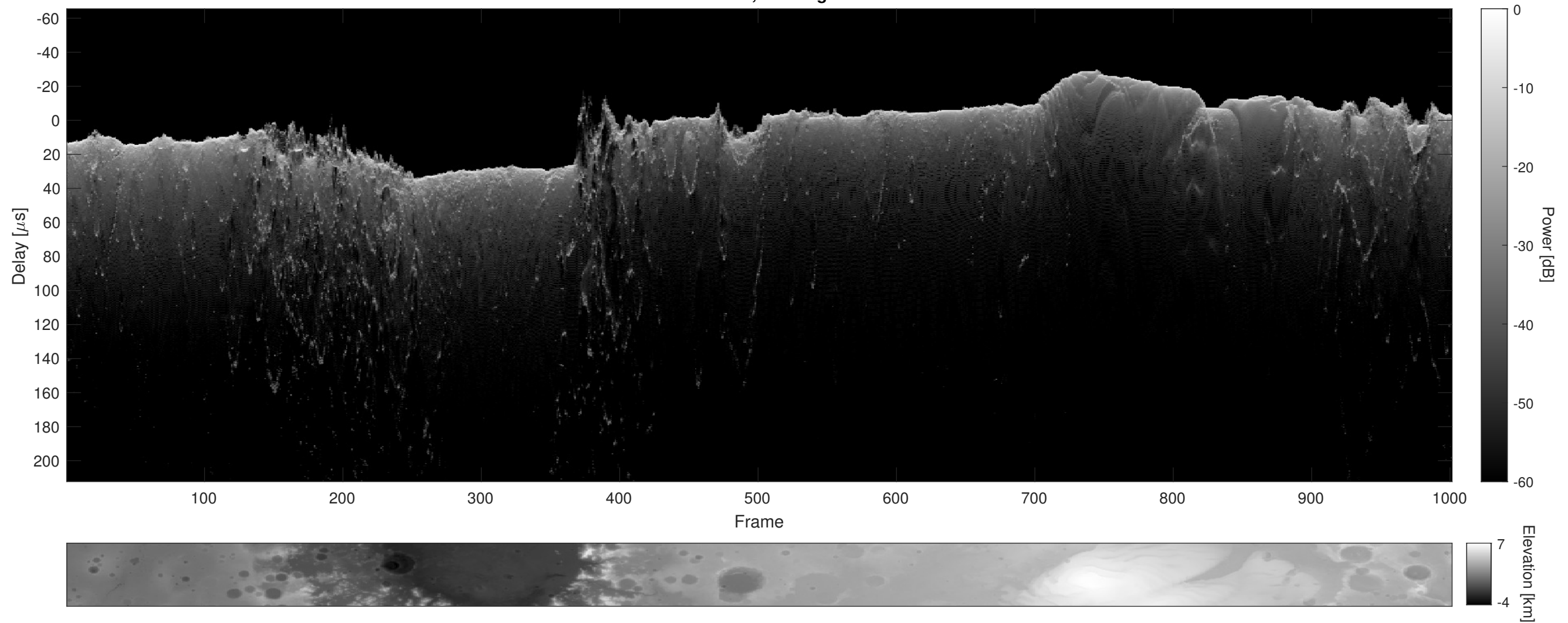
Orbit 21404, Cluttergram
