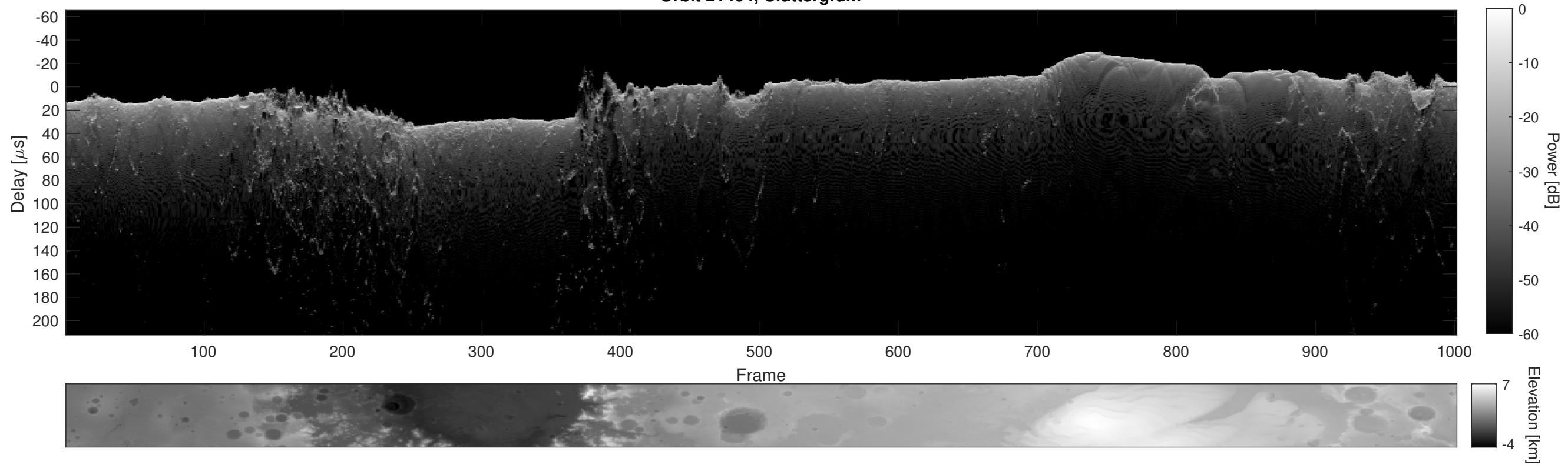
Orbit 21404, Cluttergram
