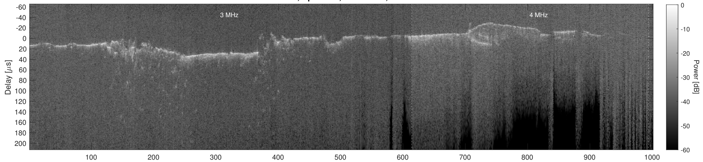
Orbit 21404, Cluttergram
