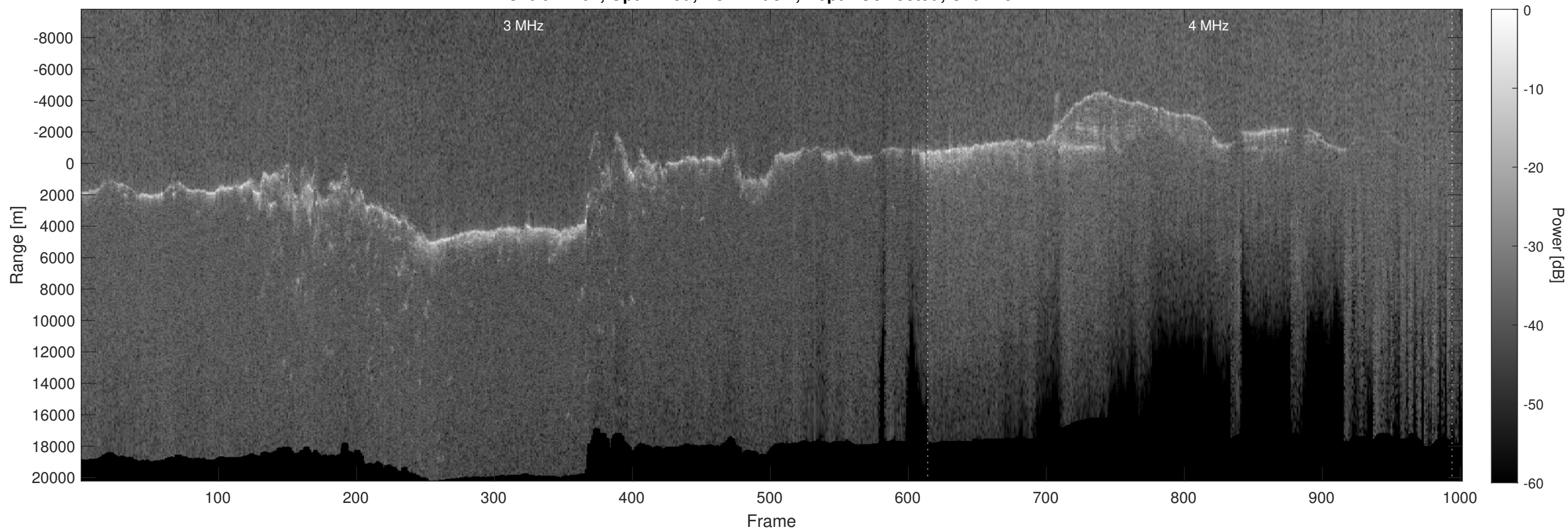
Orbit 21404, Optimized, No Window, Depth-Corrected, Channel 2
