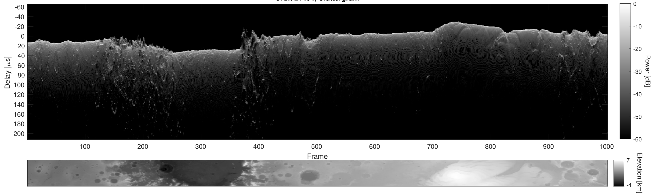
Orbit 21404, Cluttergram
