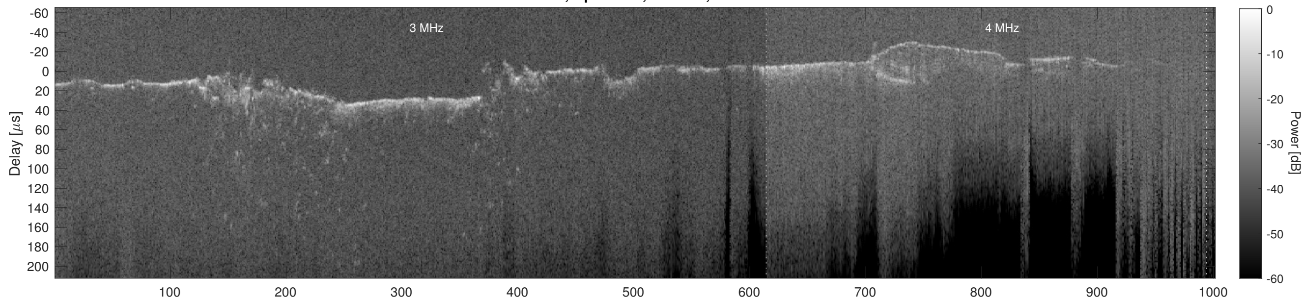
Orbit 21404, Cluttergram
