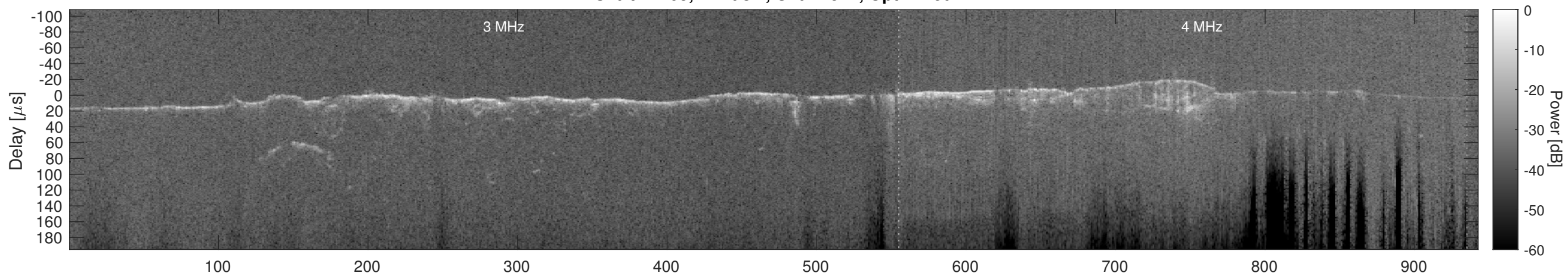
Orbit 21405, Cluttergram
