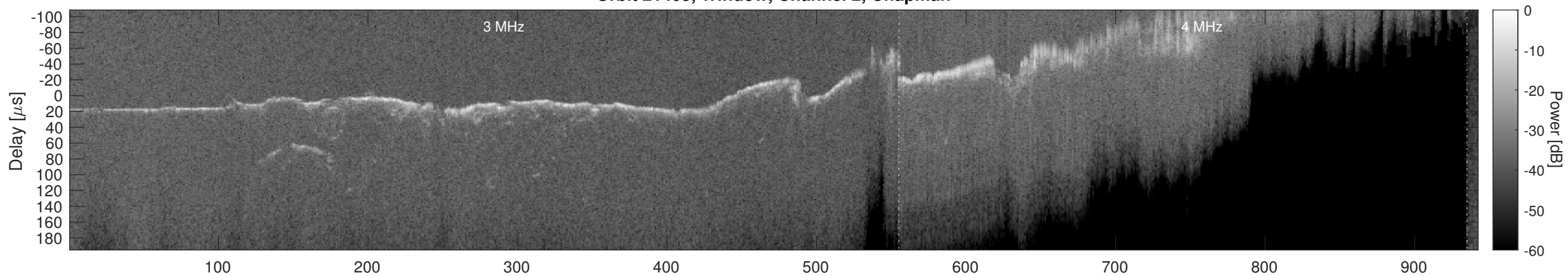
Orbit 21405, Window, Channel 2, Optimized
