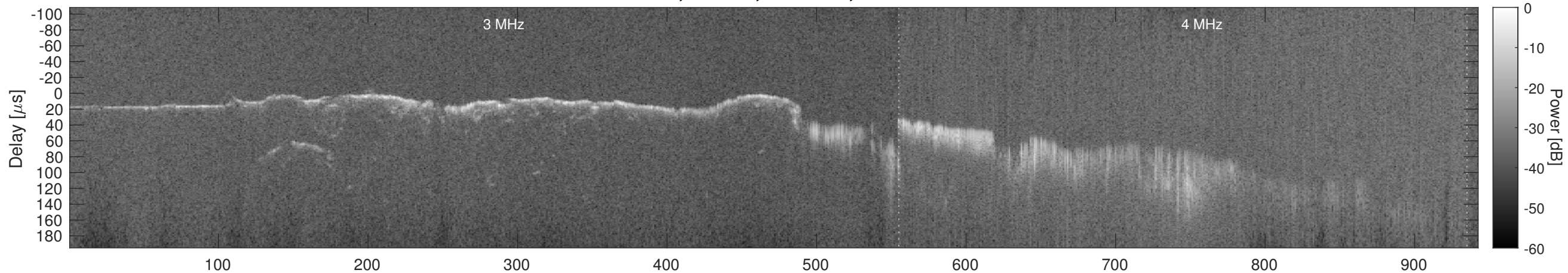
Orbit 21405, Window, Channel 2, Chapman
