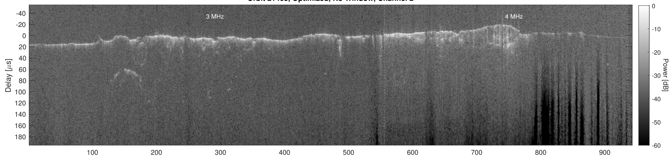
Orbit 21405, Cluttergram
