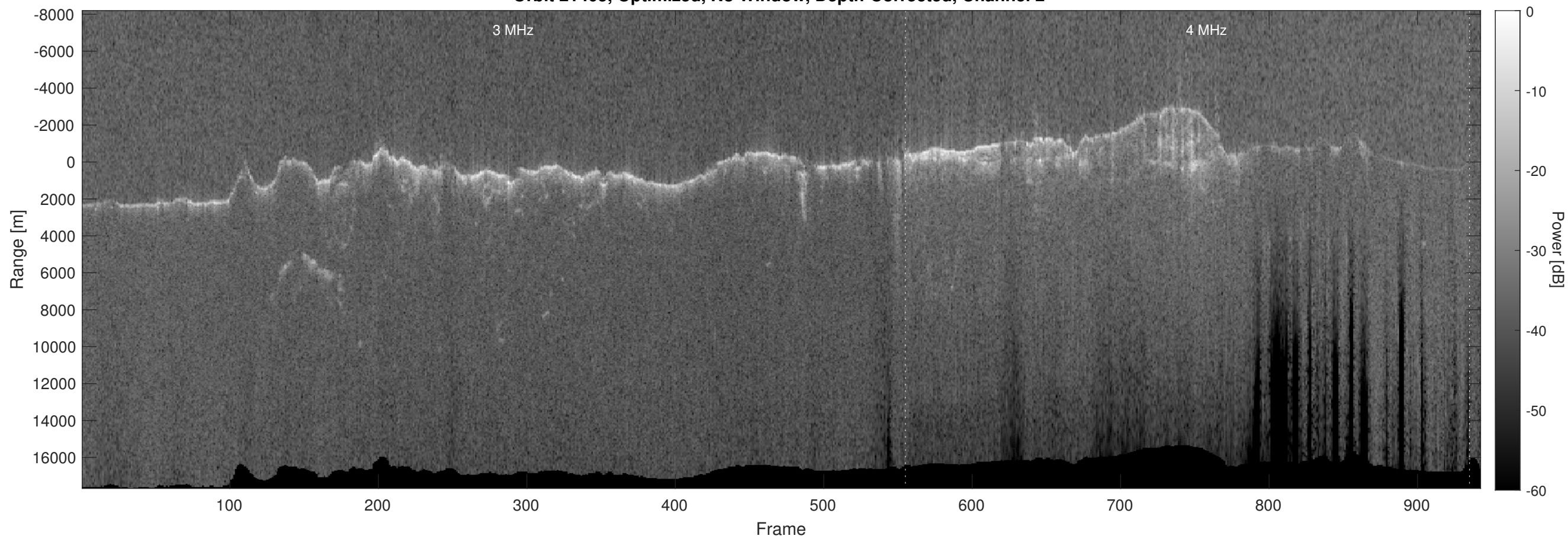
Orbit 21405, Optimized, No Window, Depth-Corrected, Channel 2
