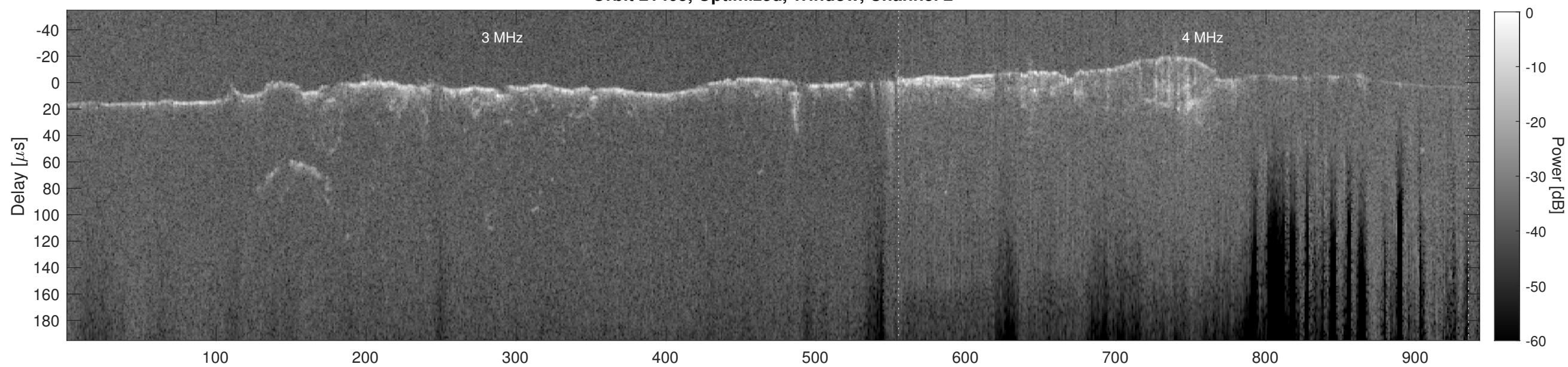
Orbit 21405, Cluttergram
