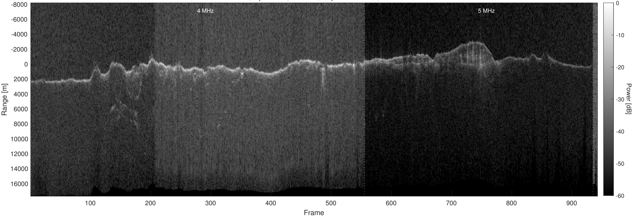
Orbit 21405, Optimized, Window, Depth-Corrected, Channel 2
