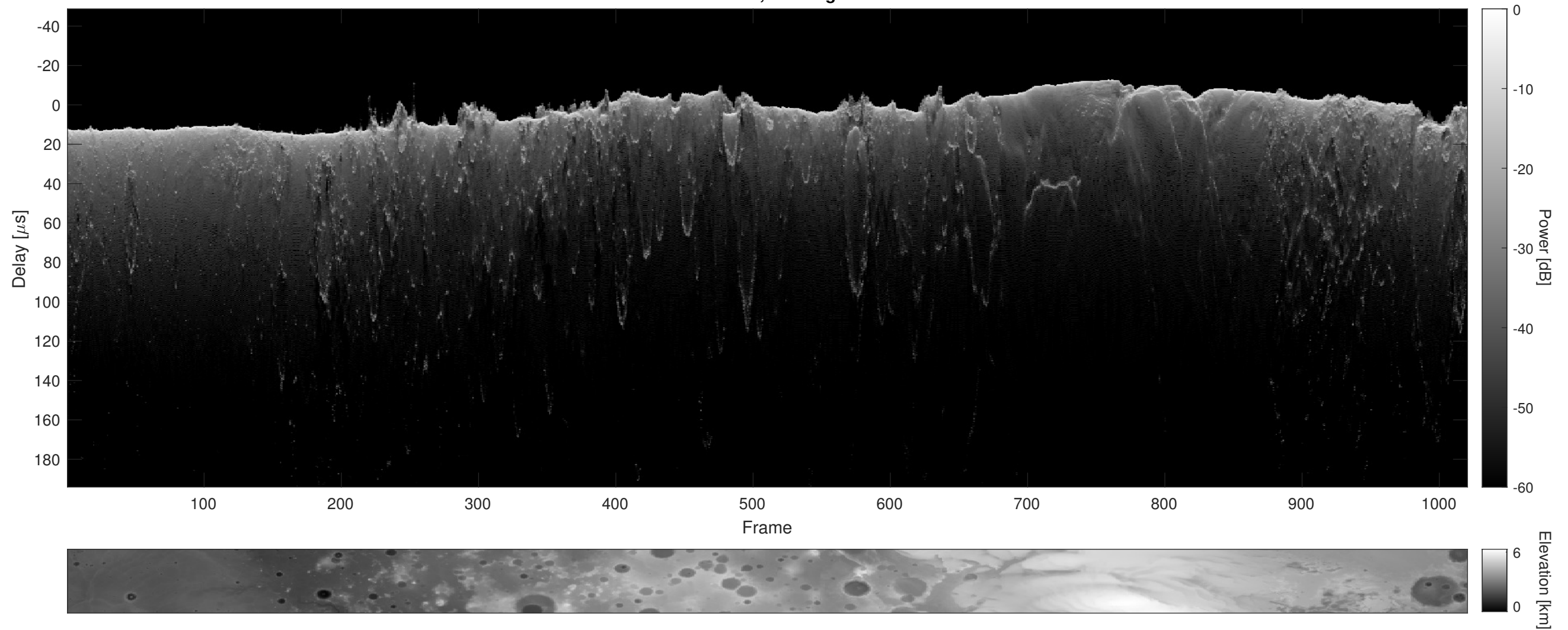
Orbit 21413, Cluttergram
