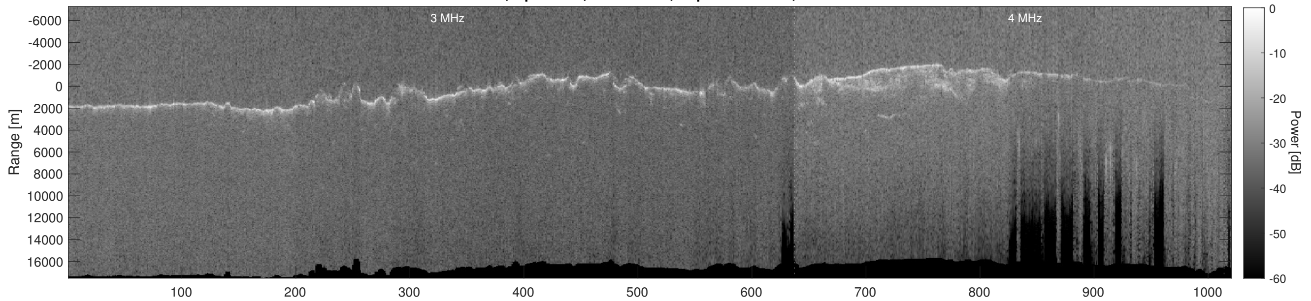
Orbit 21413, Depth-Corrected Cluttergram
