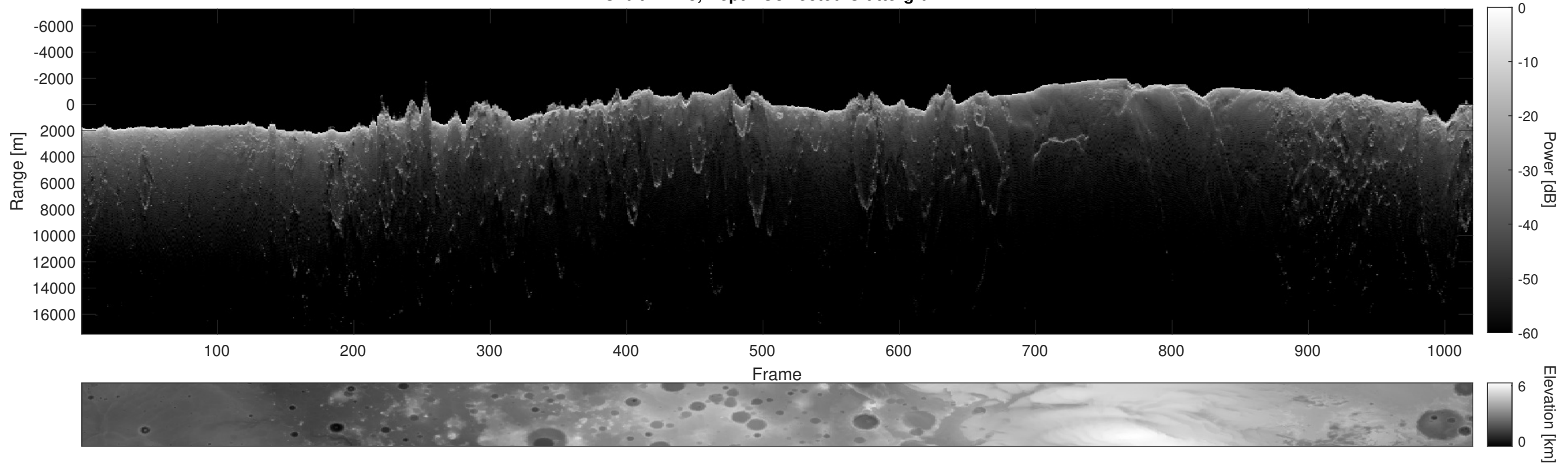
Orbit 21413, Depth-Corrected Cluttergram
