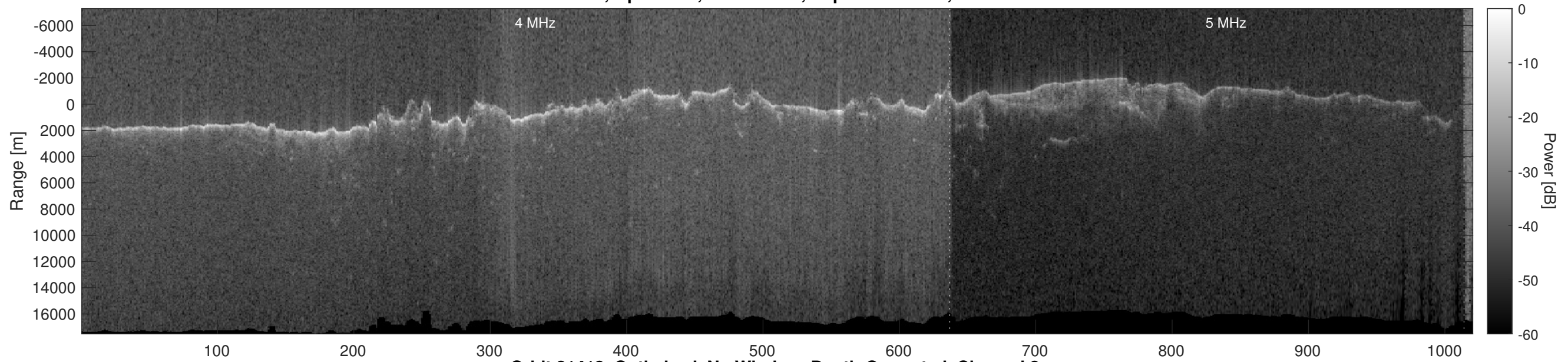
Orbit 21413, Optimized, No Window, Depth-Corrected, Channel 2
