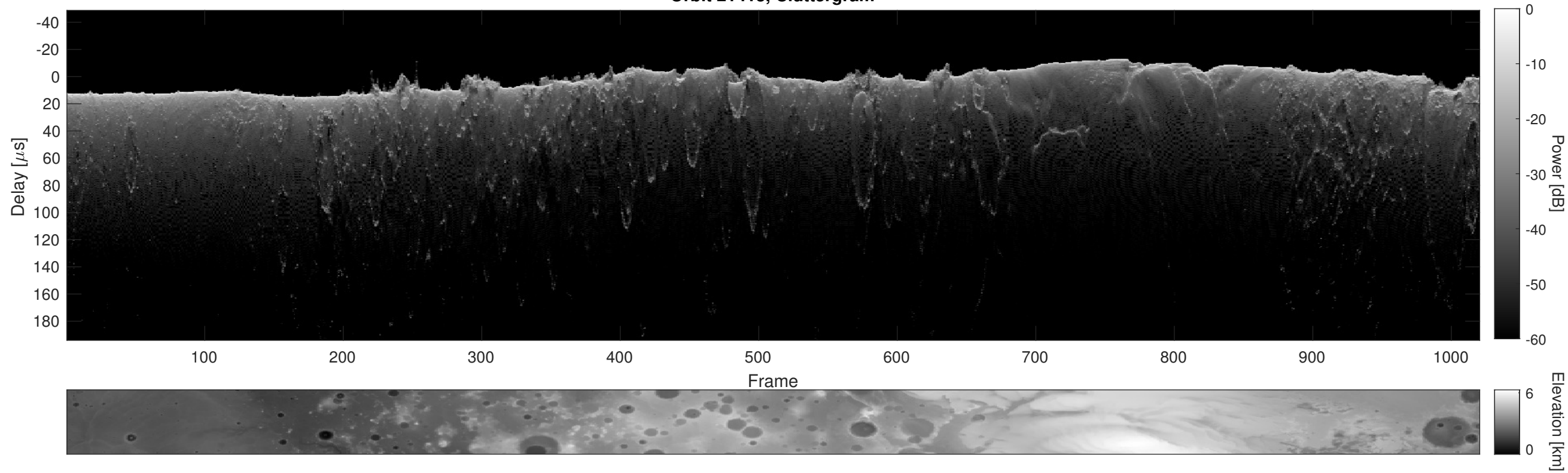
Orbit 21413, Cluttergram
