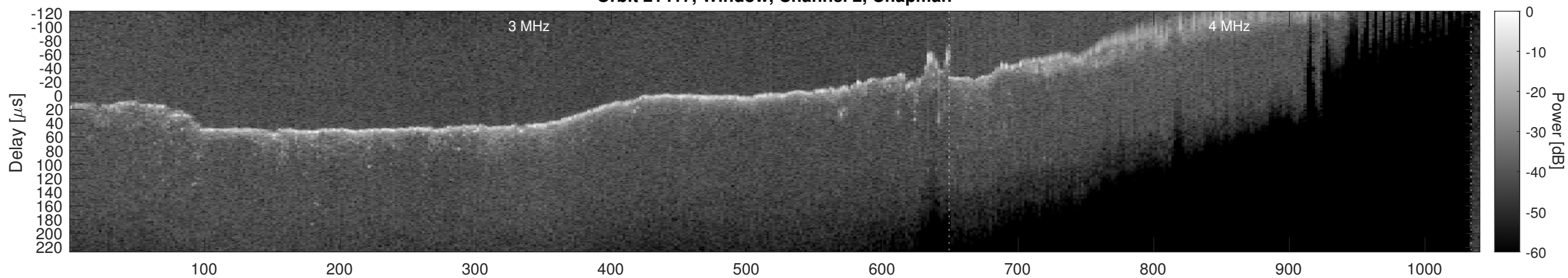
Orbit 21417, Window, Channel 2, Optimized
