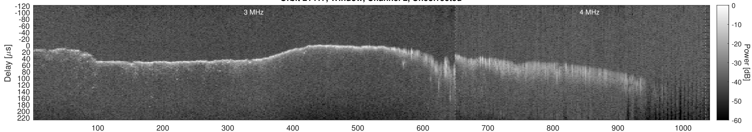
Orbit 21417, Window, Channel 2, Chapman
