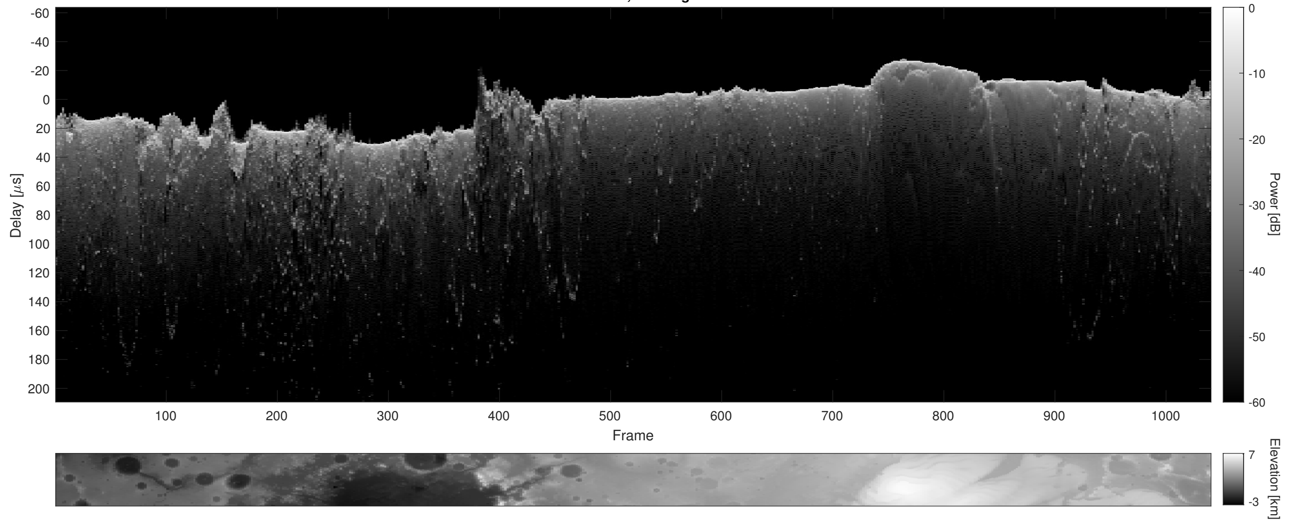
Orbit 21418, Cluttergram
