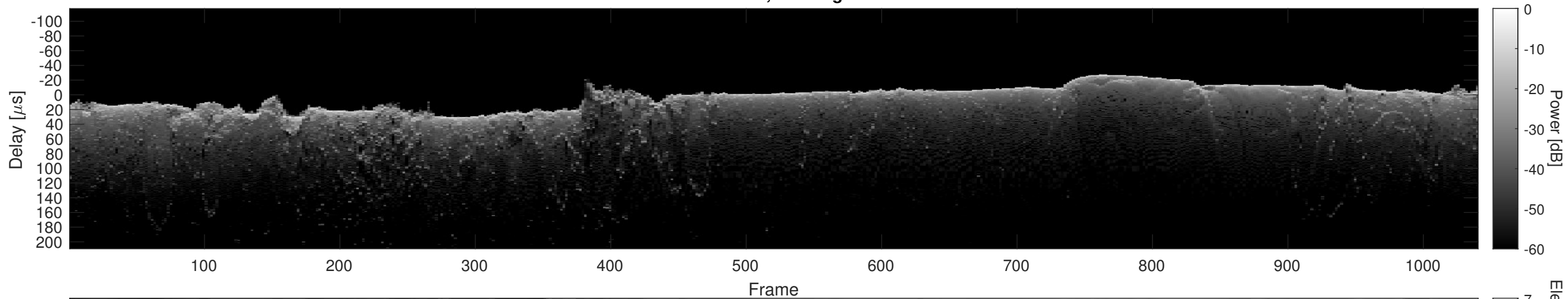
Orbit 21418, Cluttergram
