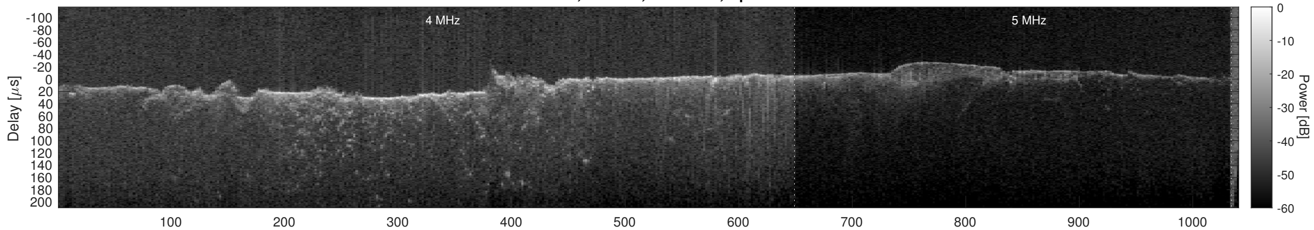
Orbit 21418, Cluttergram
