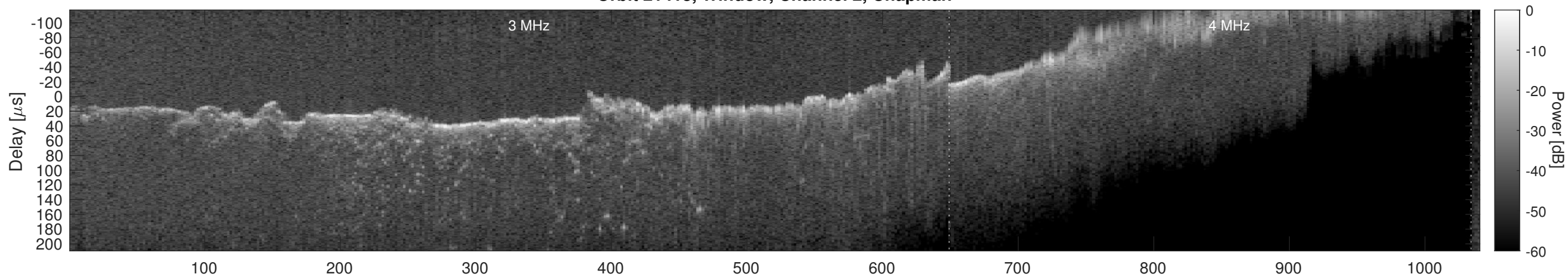
Orbit 21418, Window, Channel 2, Optimized
