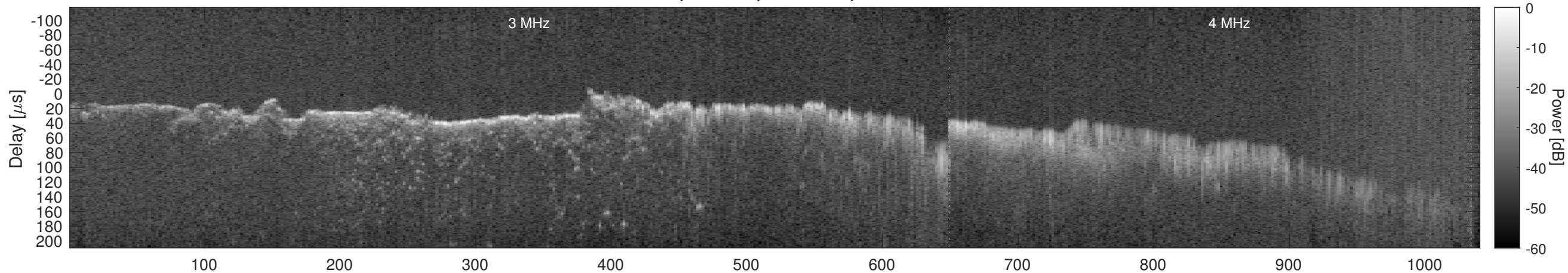
Orbit 21418, Window, Channel 2, Chapman
