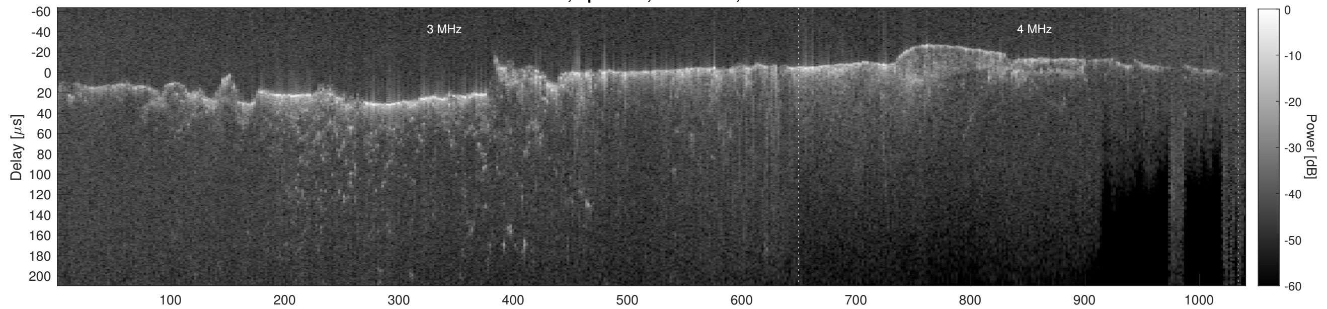
Orbit 21418, Cluttergram
