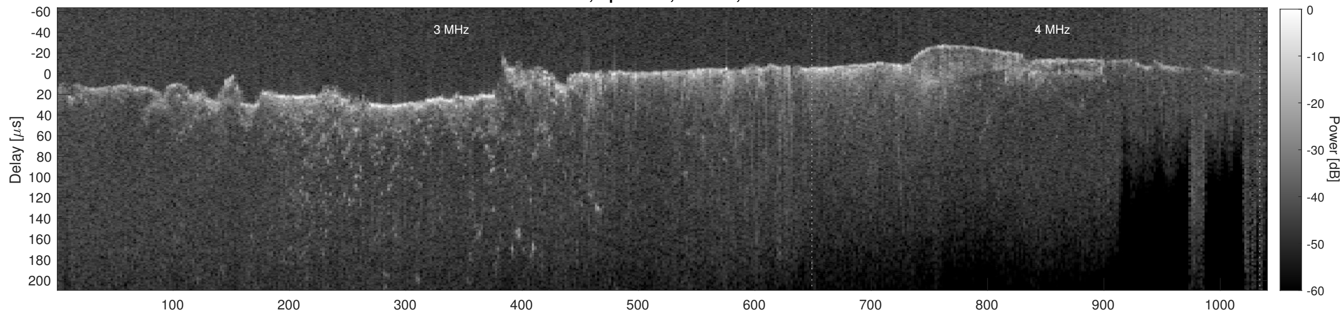
Orbit 21418, Cluttergram
