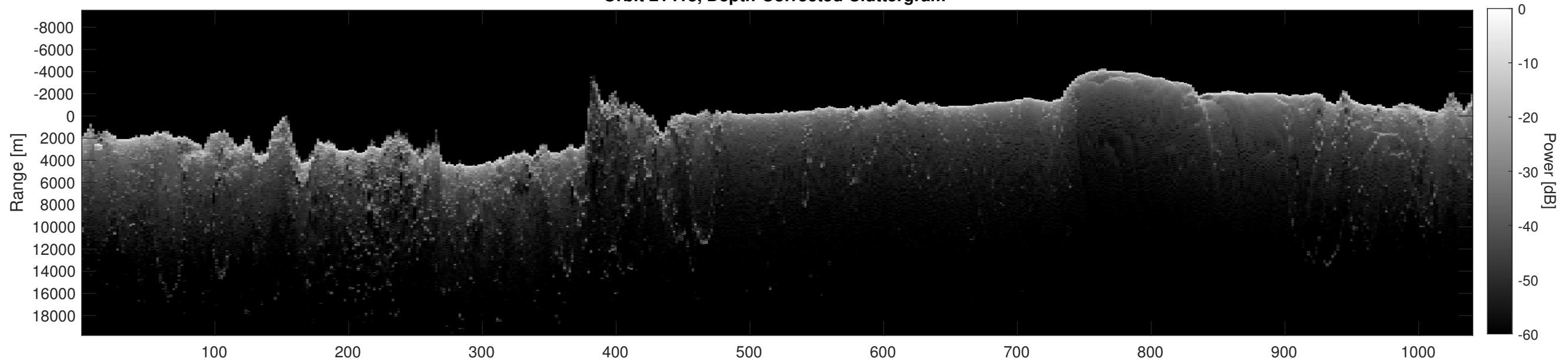
Orbit 21418, Depth-Corrected Cluttergram
