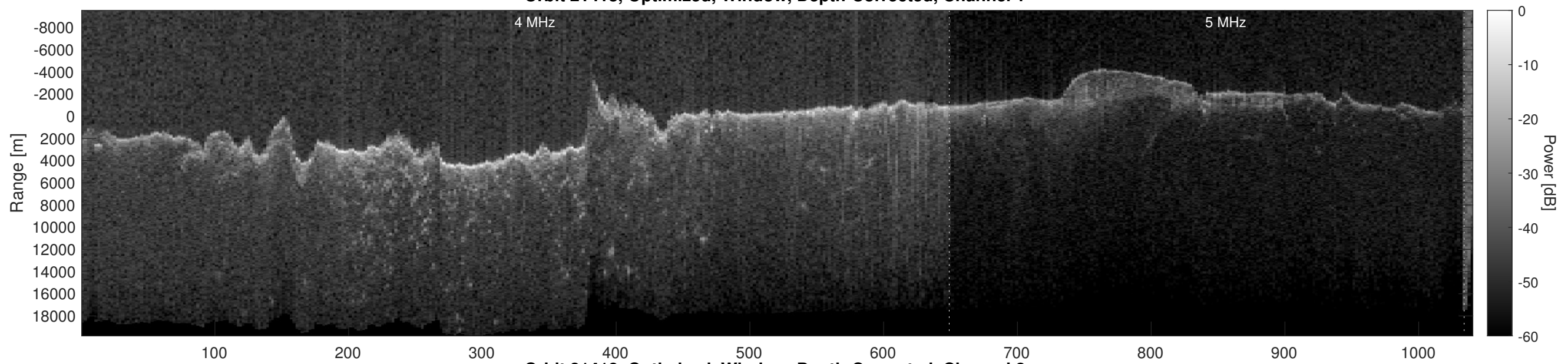
Orbit 21418, Optimized, Window, Depth-Corrected, Channel 2
