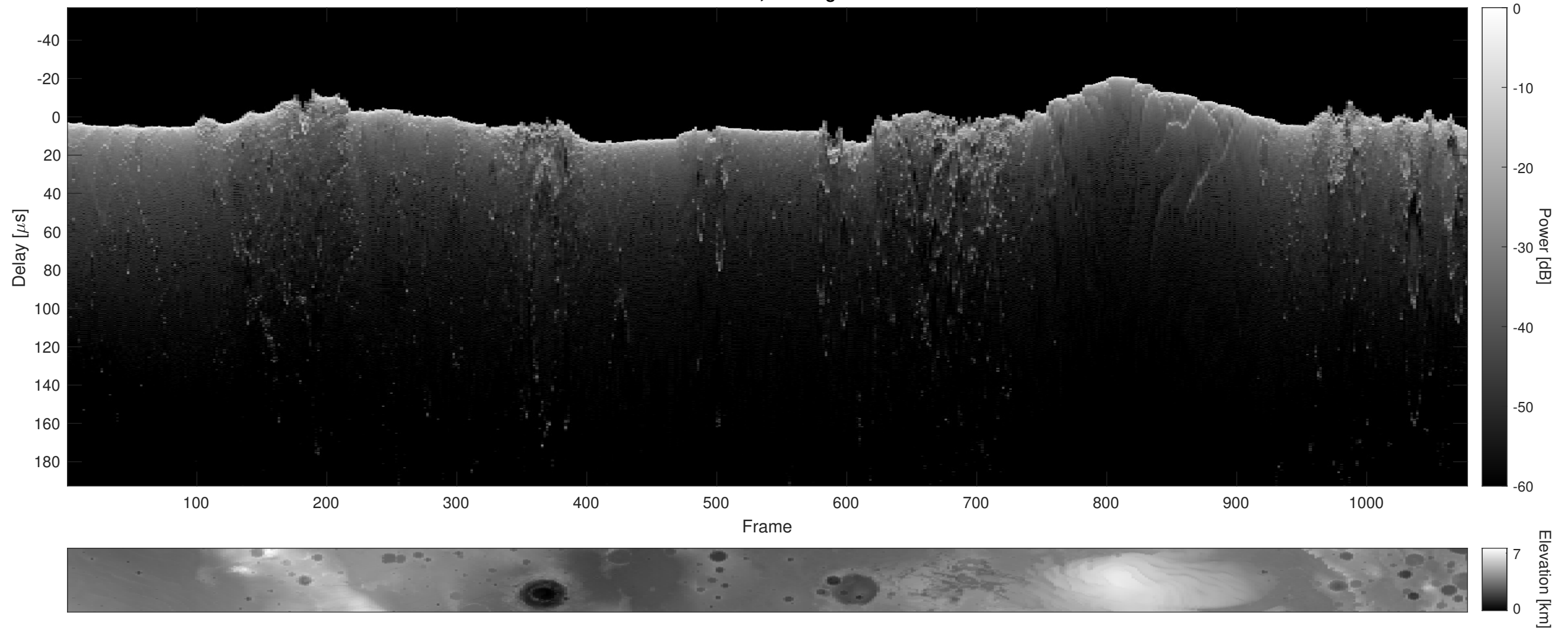
Orbit 21429, Cluttergram
