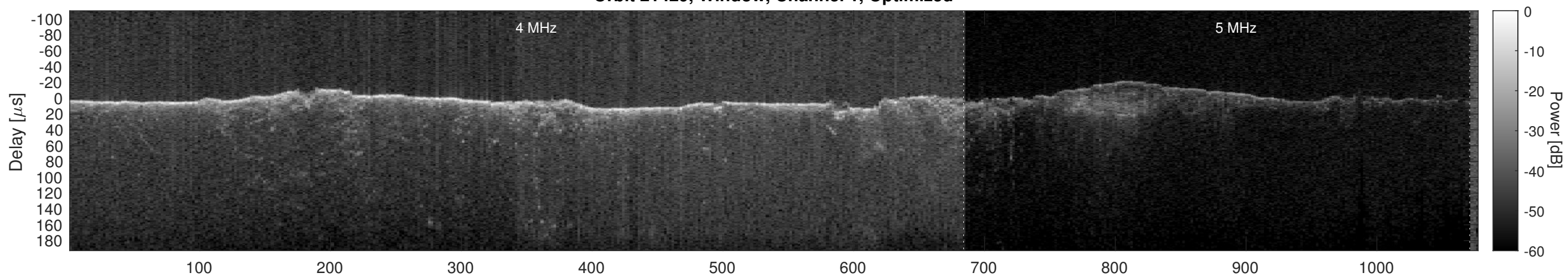
Orbit 21429, Cluttergram
