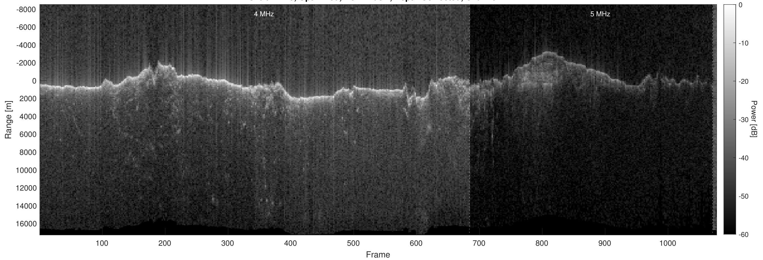
Orbit 21429, Optimized, No Window, Depth-Corrected, Channel 2
