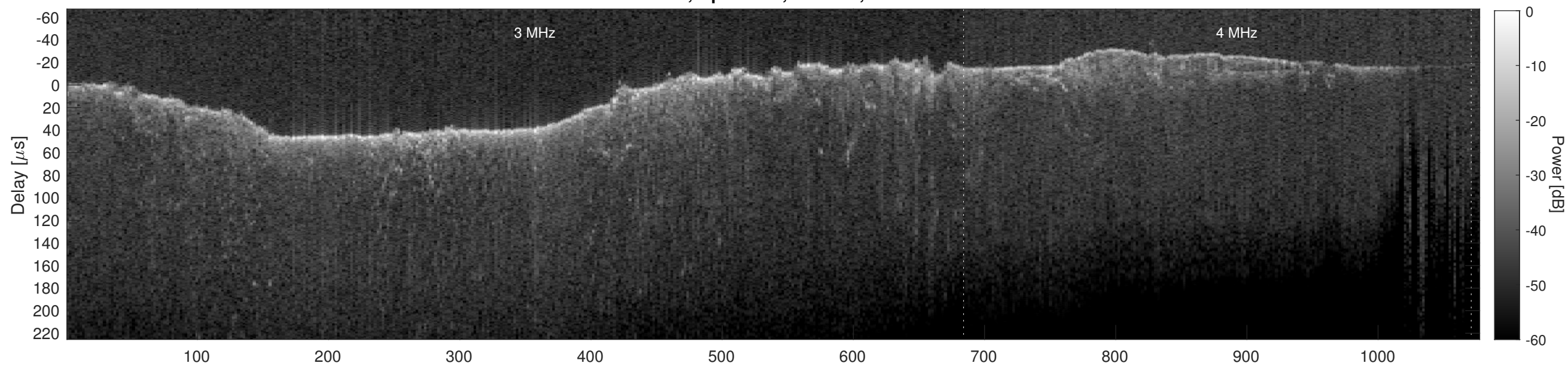
Orbit 21431, Cluttergram
