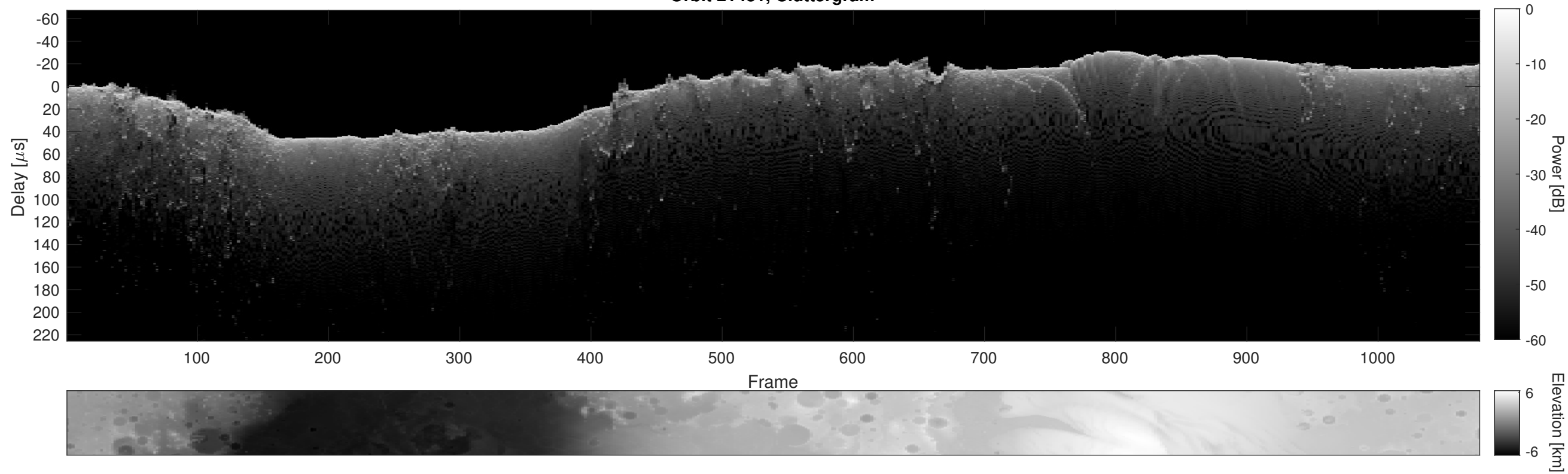
Orbit 21431, Cluttergram
