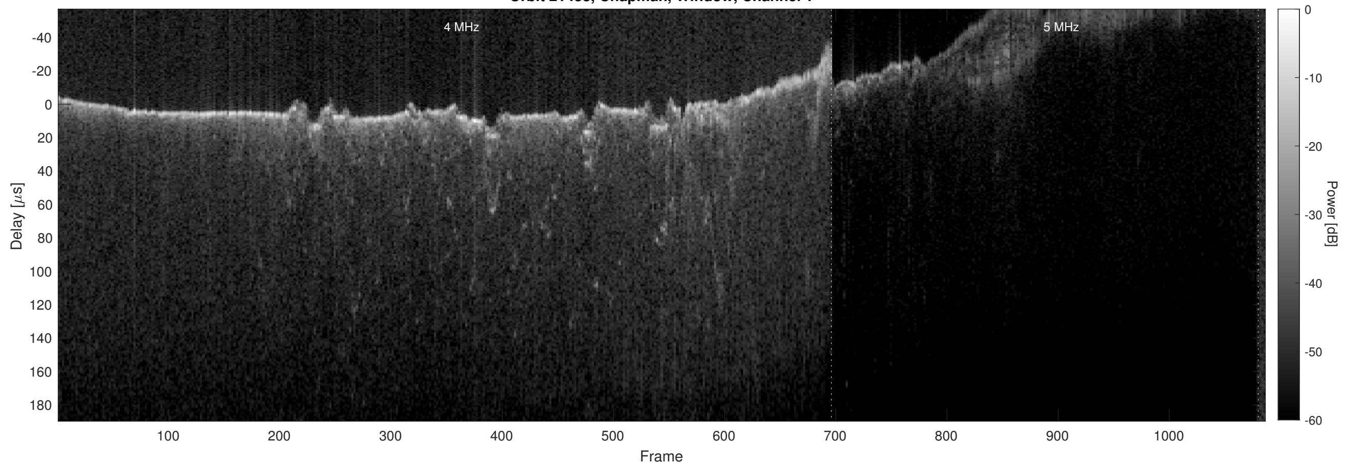
Orbit 21433, Chapman, Window, Channel 2
