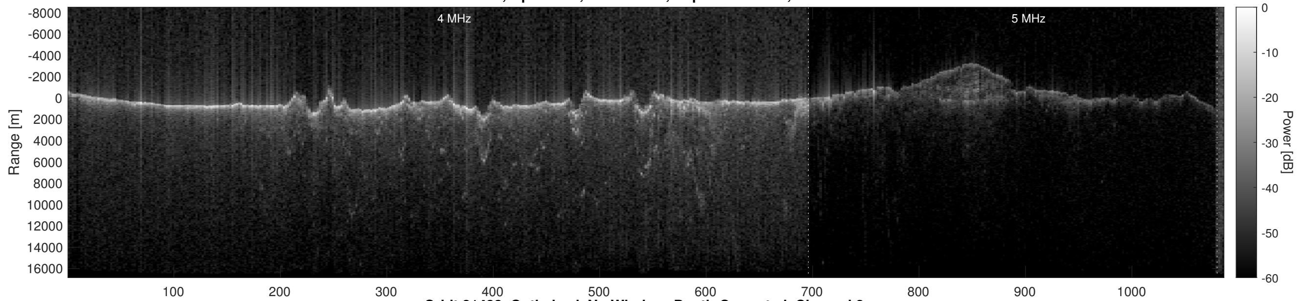
Orbit 21433, Optimized, No Window, Depth-Corrected, Channel 2
