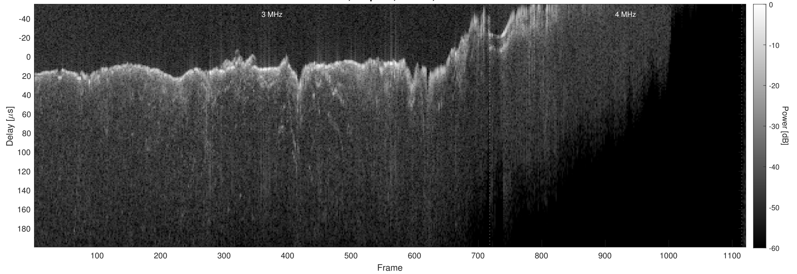
Orbit 21444, Chapman, Window, Channel 2
