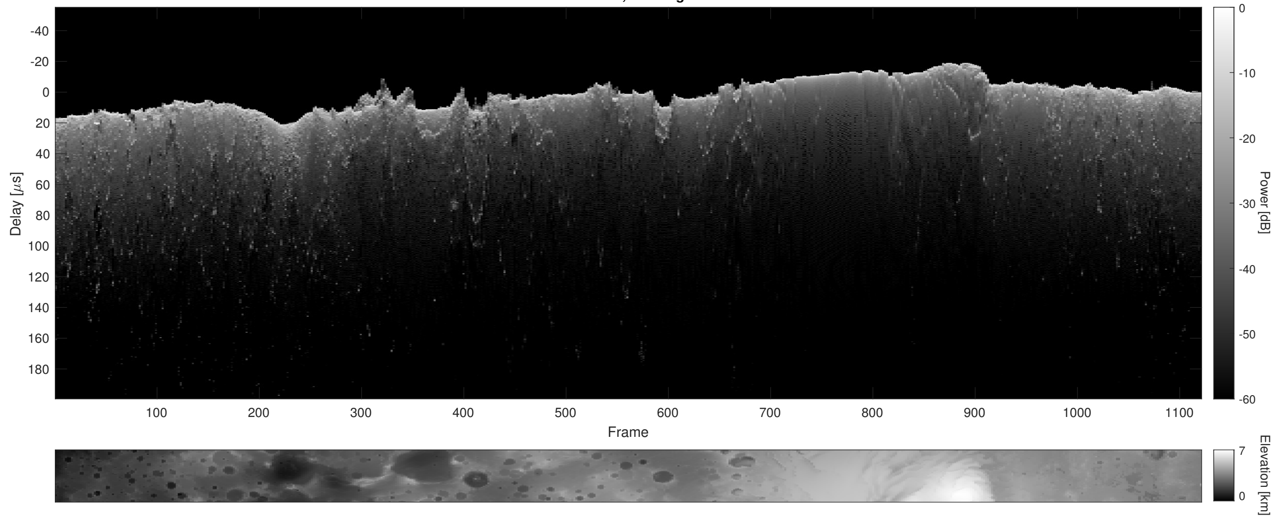
Orbit 21444, Cluttergram
