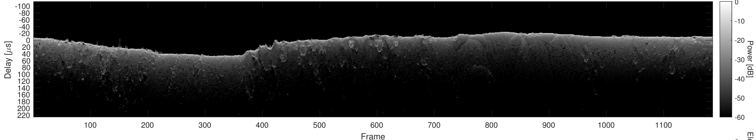
Orbit 21445, Cluttergram
