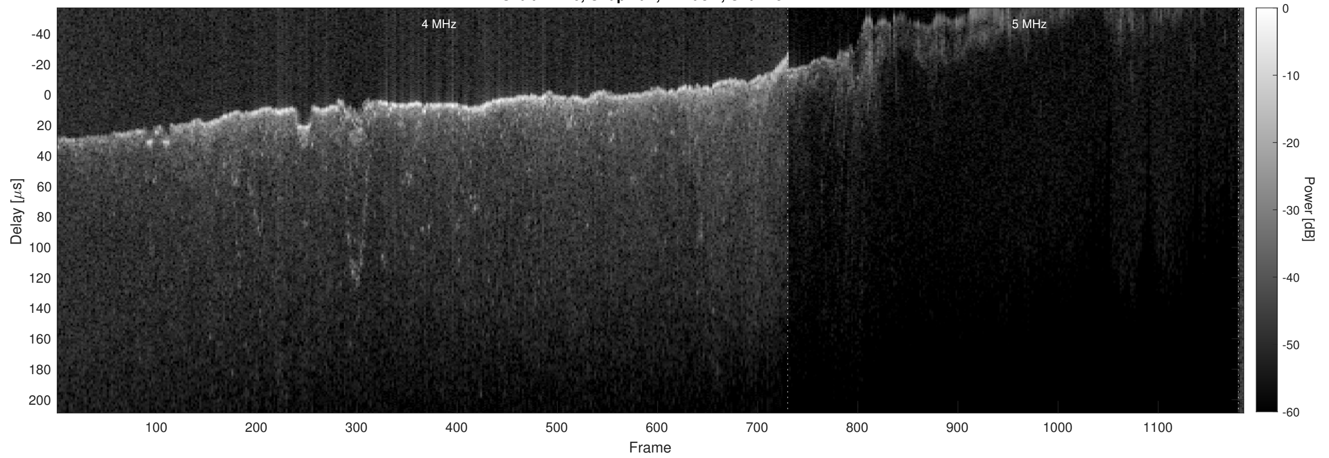
Orbit 21446, Chapman, Window, Channel 2
