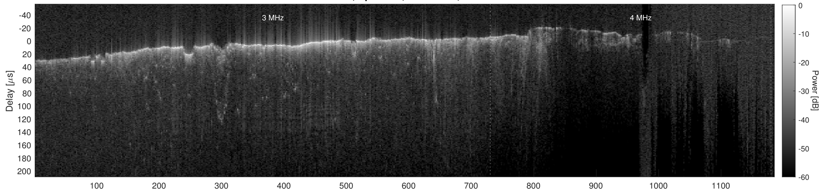
Orbit 21446, Cluttergram
