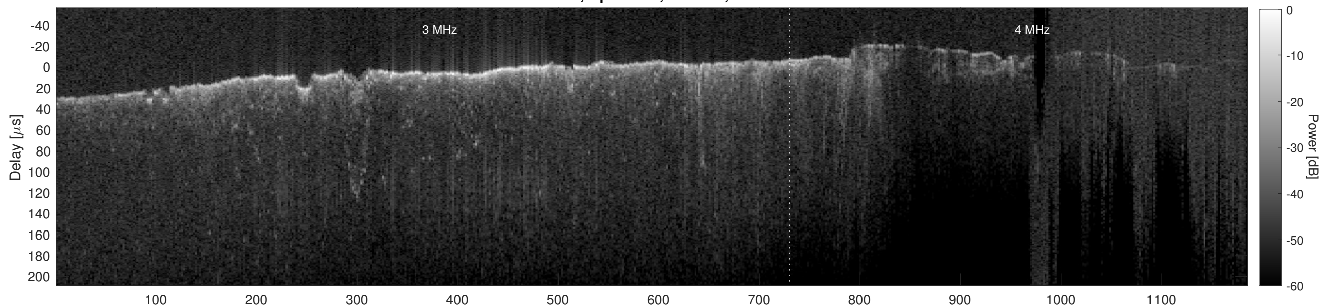
Orbit 21446, Cluttergram
