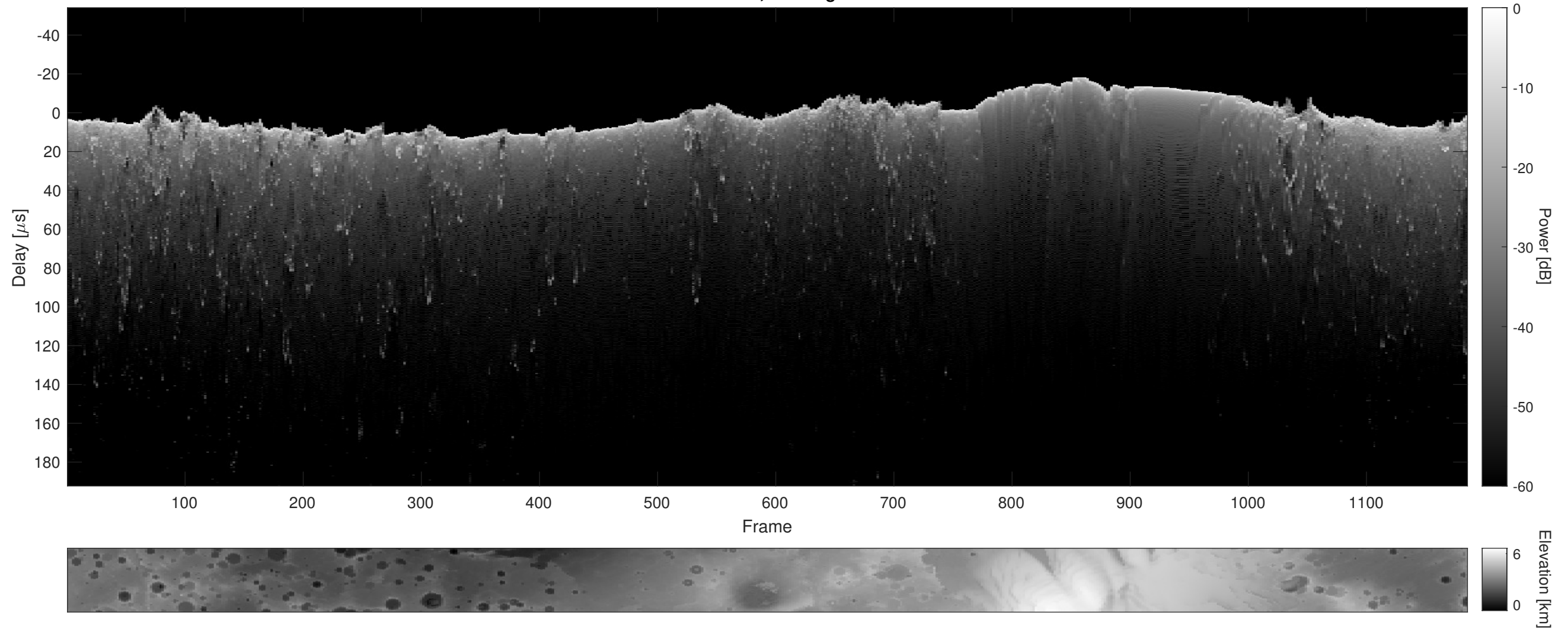
Orbit 21449, Cluttergram
