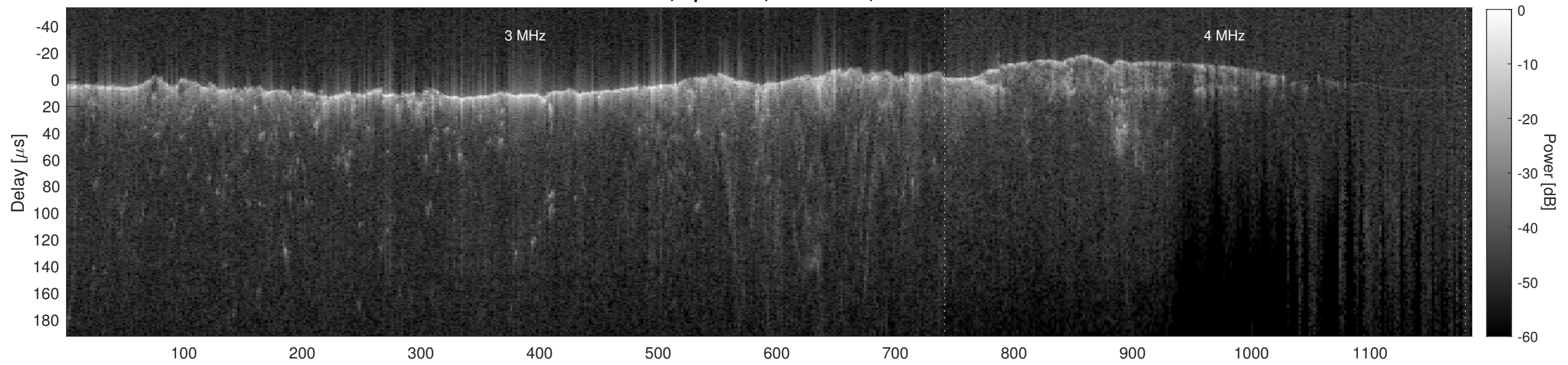
Orbit 21449, Cluttergram
