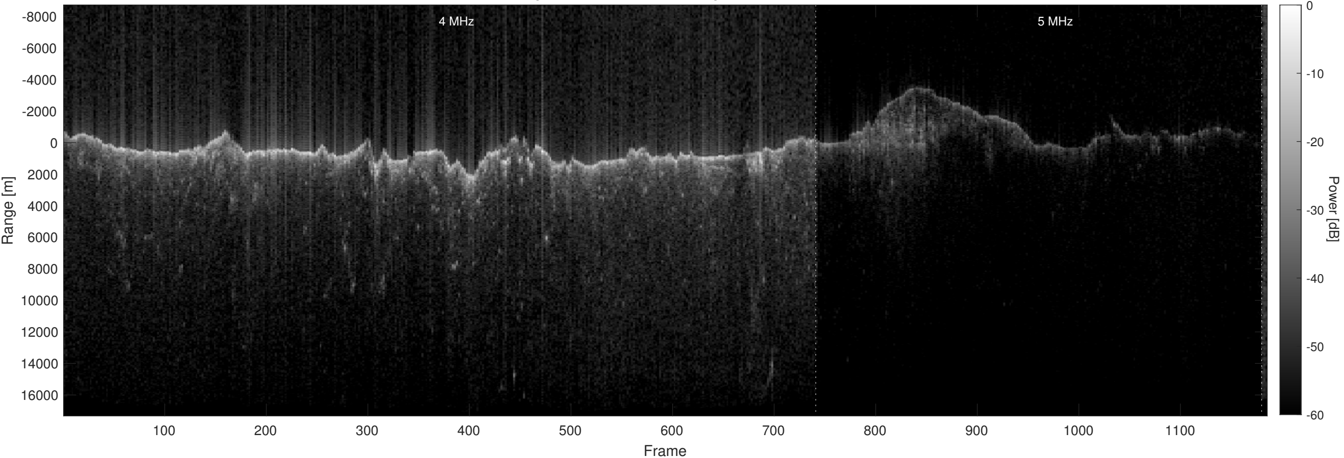
Orbit 21450, Optimized, No Window, Depth-Corrected, Channel 2
