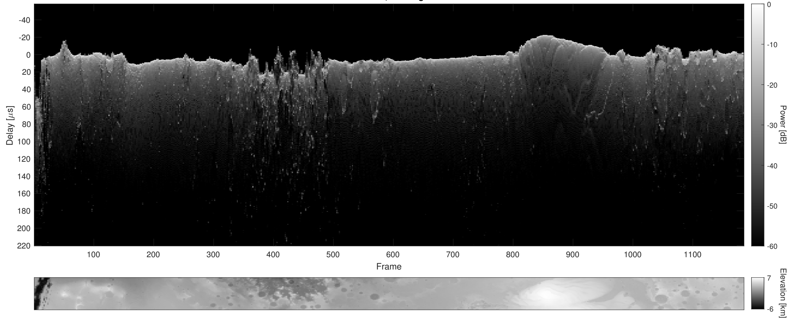
Orbit 21457, Cluttergram
