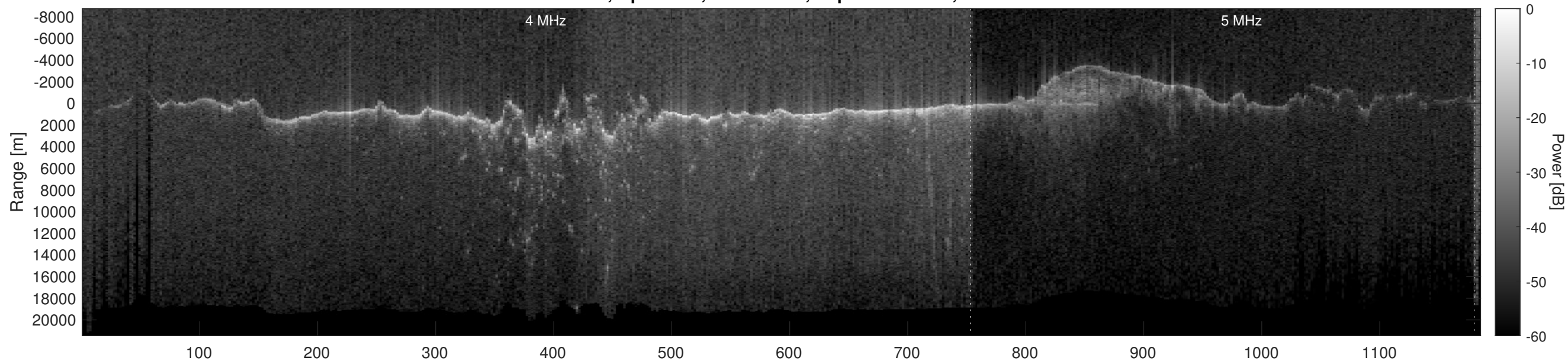
Orbit 21457, Optimized, No Window, Depth-Corrected, Channel 2
