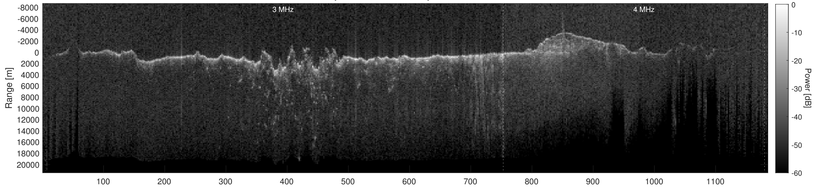
Orbit 21457, Depth-Corrected Cluttergram
