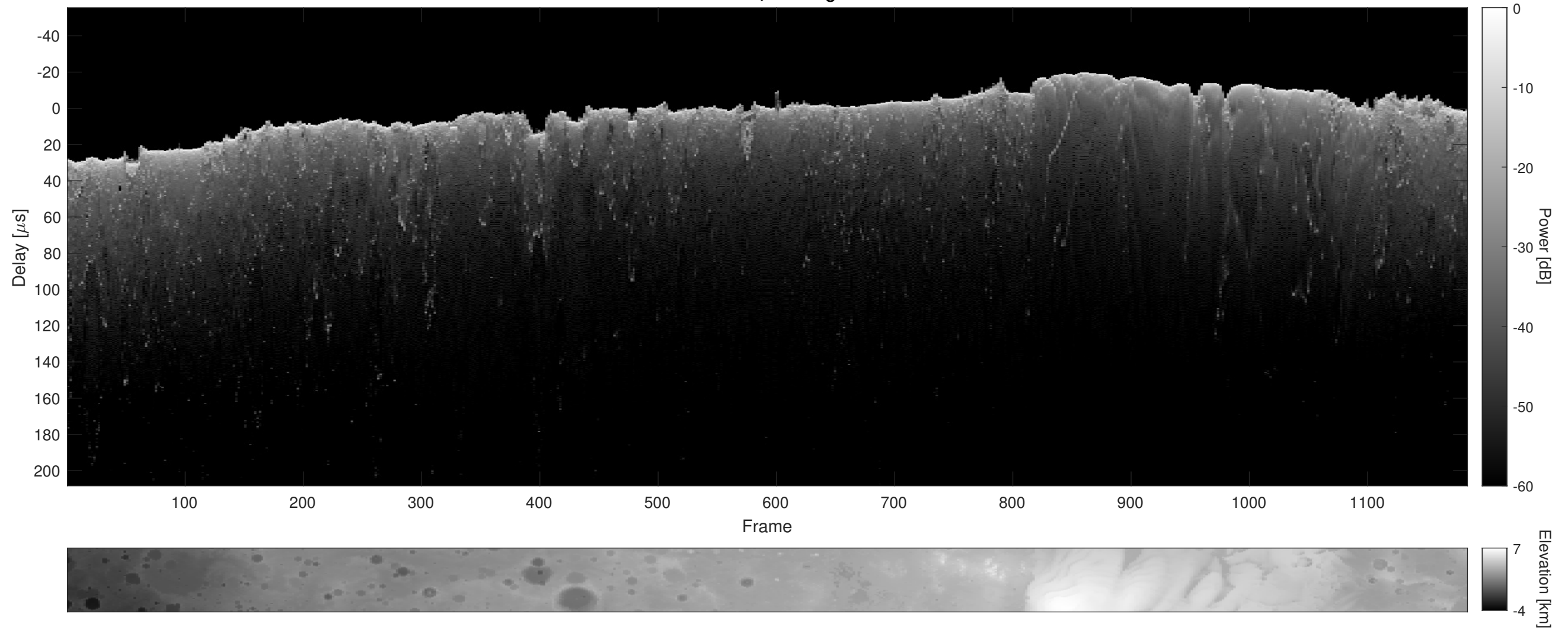
Orbit 21460, Cluttergram
