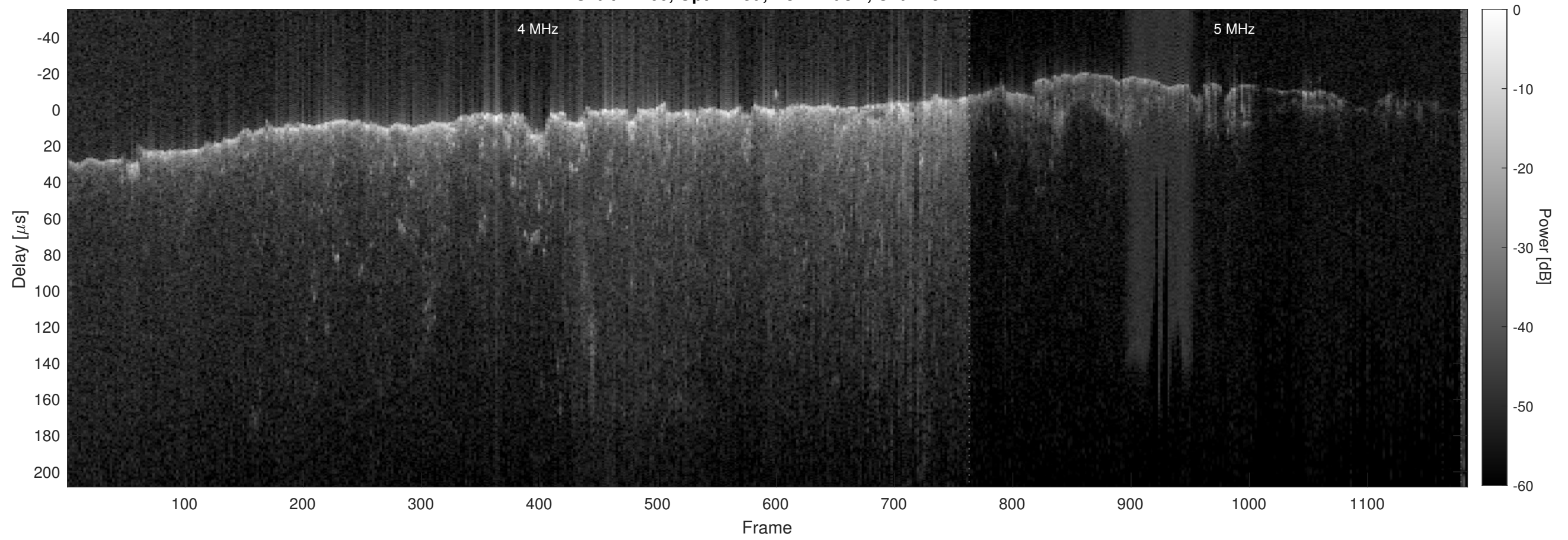
Orbit 21460, Optimized, No Window, Channel 2
