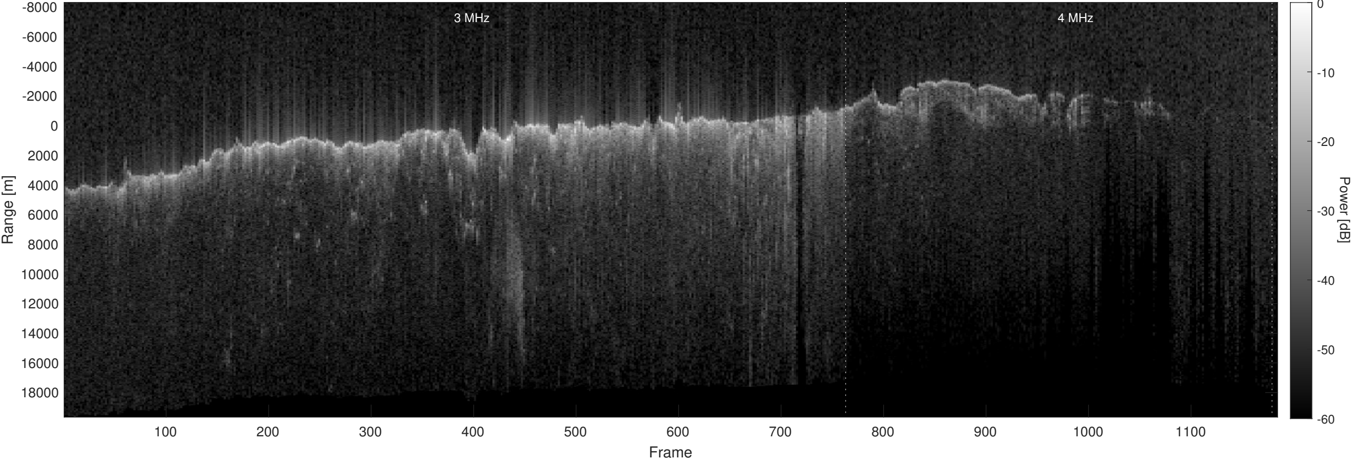
Orbit 21460, Optimized, No Window, Depth-Corrected, Channel 2
