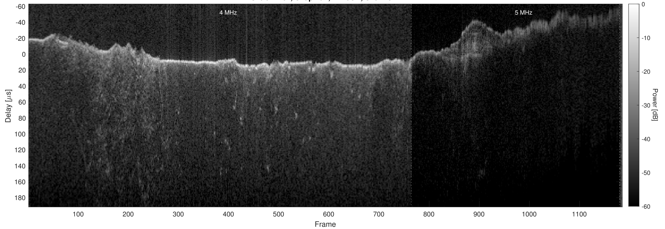
Orbit 21461, Chapman, Window, Channel 2
