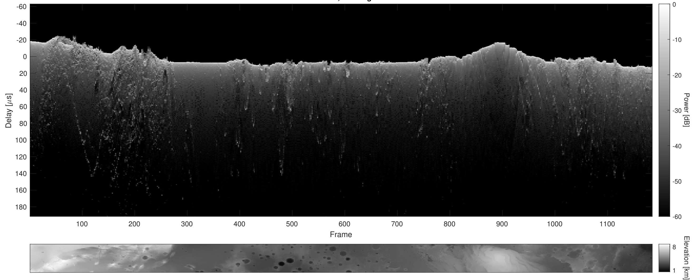
Orbit 21461, Cluttergram
