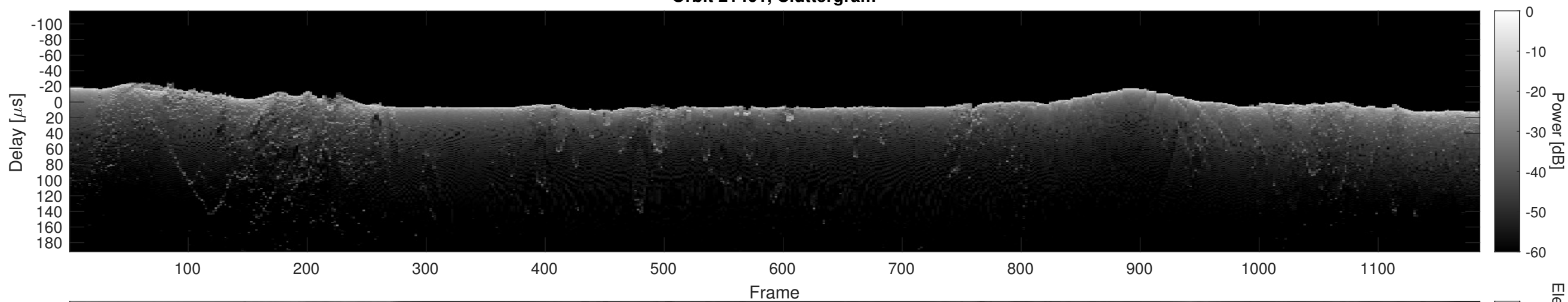
Orbit 21461, Cluttergram
