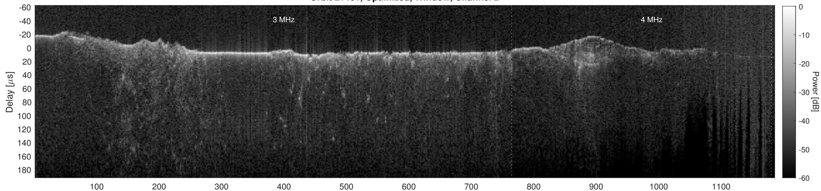
Orbit 21461, Cluttergram
