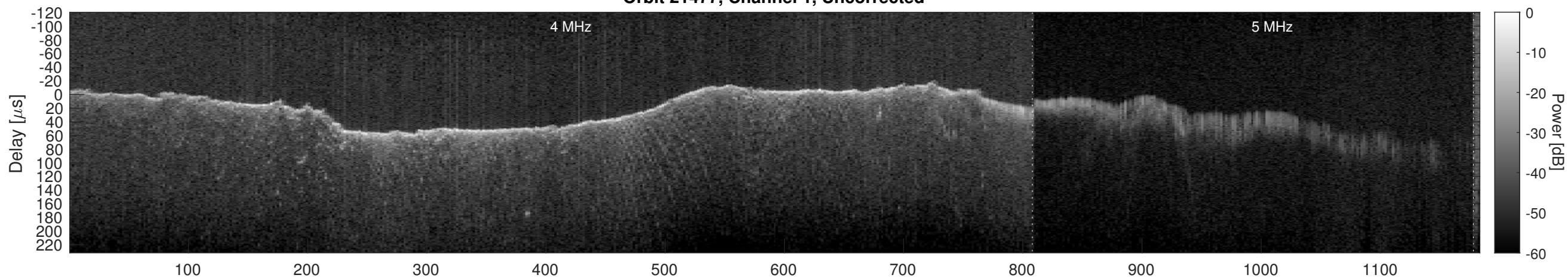
Orbit 21477, Window, Channel 1, Chapman
