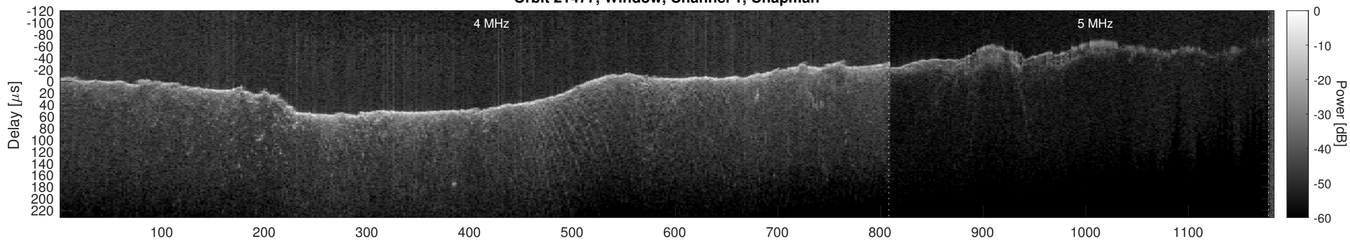
Orbit 21477, Window, Channel 1, Optimized
